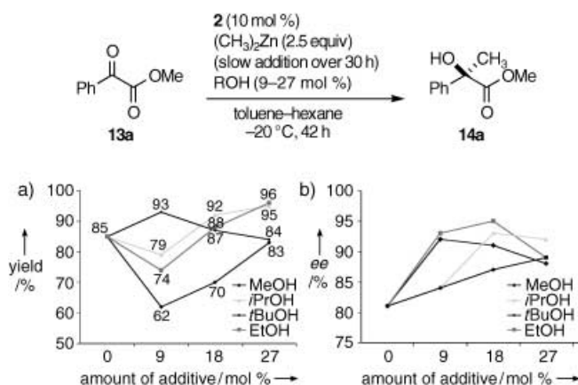
Figure 2. Effect of additive alcohol on yield and enantioselectivity. a) Relationship between yield and amount of additive. b) Relationship between ee and amount of additive.
