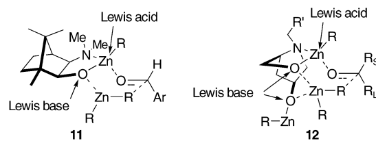
Figure 1. Fundamental concepts of catalyst design.
